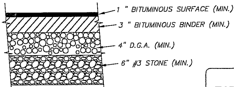
PAVEMENT DETAIL NO SCALE
